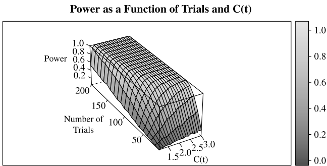
Fig. 4. Power of the U_{OR} and U_{AND} statistics with \alpha = 0.05 as a function of capacity and number of trials per distribution for capacity above 1. These results are based on two exponential channels, with either an OR or AND stopping rule, depending on the statistic. Using these models, the power of U_{OR} and U_{AND} is the same.
