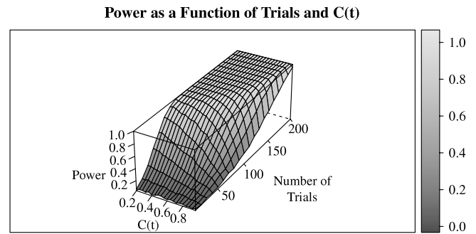
Fig. 5. Power of the U_{OR} and U_{AND} statistics with \alpha = 0.05 as a function of capacity and number of trials per distribution for capacity less than 1. These results are based on two exponential channels, with either an OR or AND stopping rule, depending on the statistic. Using these models, the power of U_{OR} and U_{AND} is the same.
