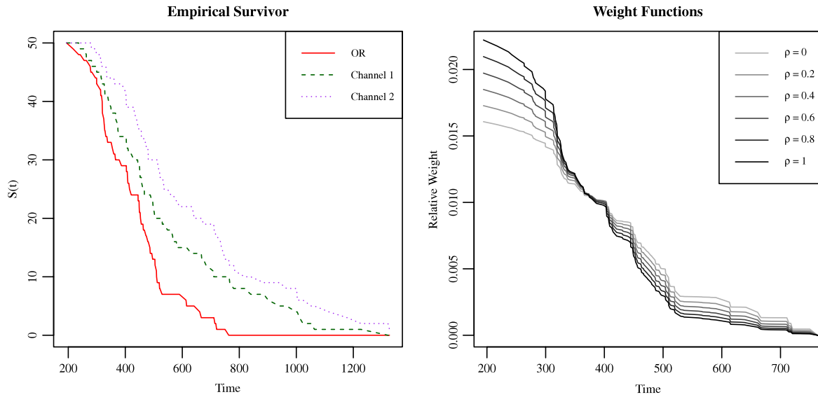
Fig. 2. On the left, the empirical survivor function based on response times sampled from Wald distributions is shown. The right shows the relative values of the Harrington–Fleming (Harrington & Fleming, 1982) weighting function for the capacity test at various values of \rho .
